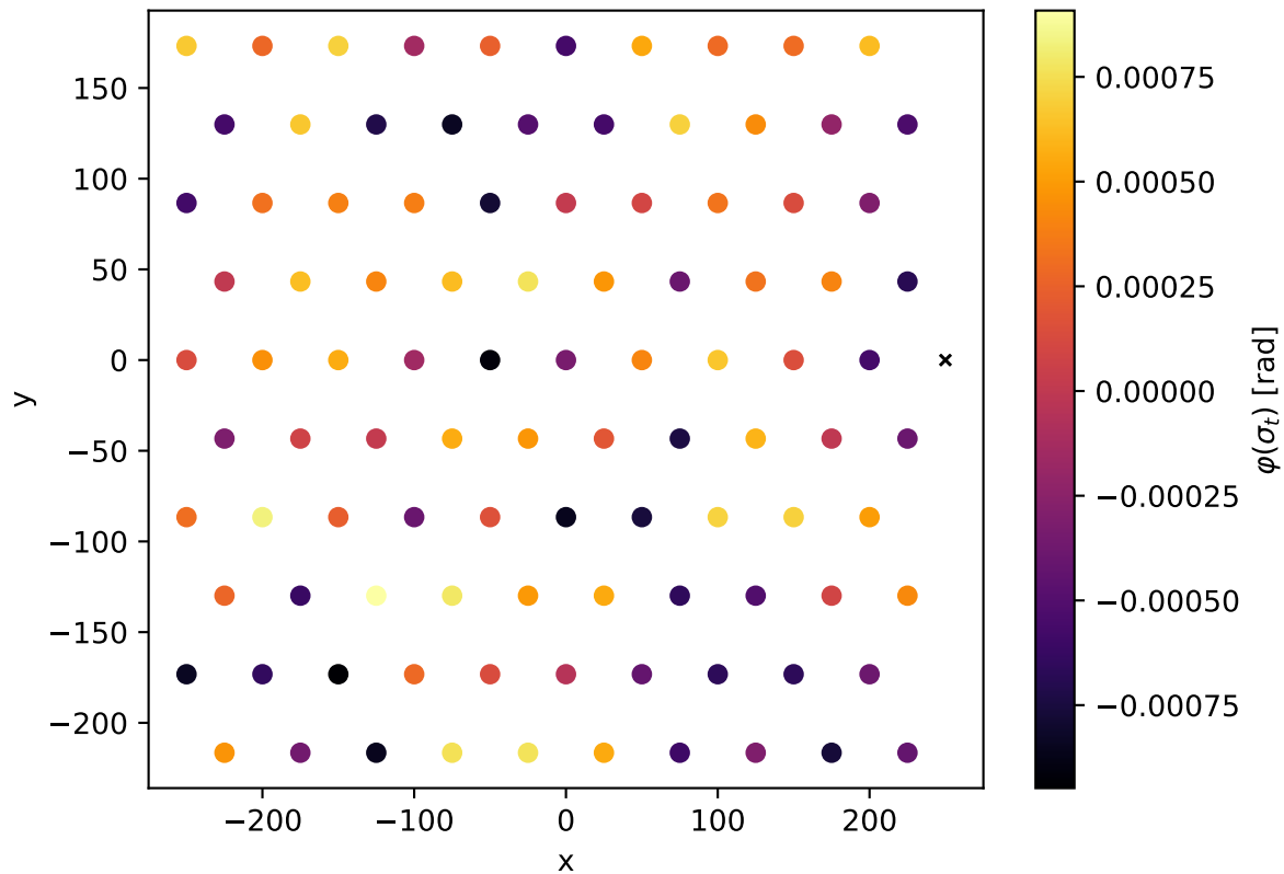
Clock phases f_beacon= 52MHz
