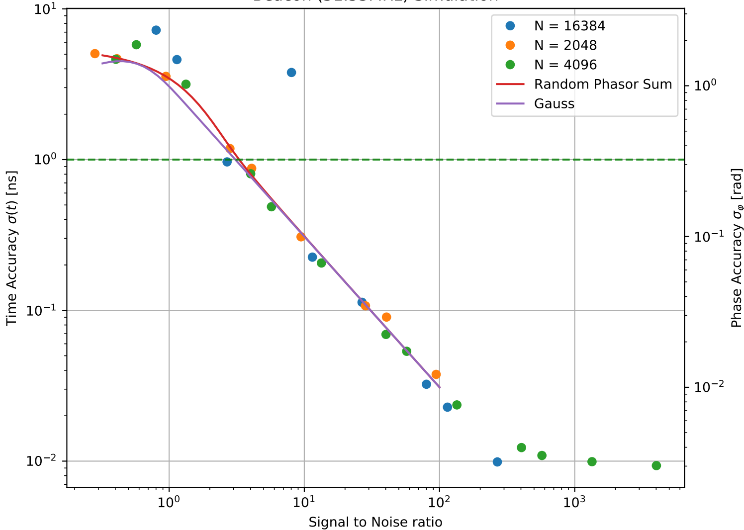
Beacon (51.53MHz) Simulation
