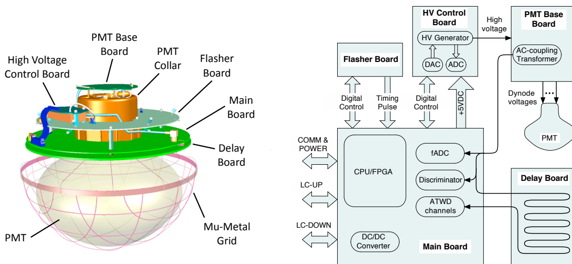
Figure 3. Components of the DOM, showing mechanical layout (left) and functional connections (right).
