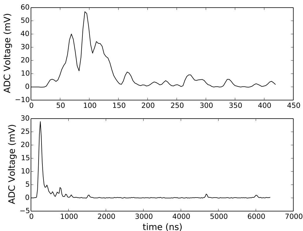
Figure 6. The same signal sampled in the ATWD (top) and the fADC (bottom): the ATWD recording duration is 427 ns whereas the fADC recording duration is 6.4 \mu s. Energy reconstruction in IceCube uses the charge and time recorded in the waveform [21].
