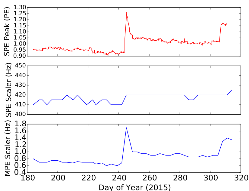
Figure 25. Mean of the Gaussian fit to the SPE peak (top) and the SPE scaler rate (middle) and MPE scaler rate (bottom) from July 2015 to November 2015 for a DOM that shows unpredictable gain shift behavior. The DOM configuration was unchanged during this period.
