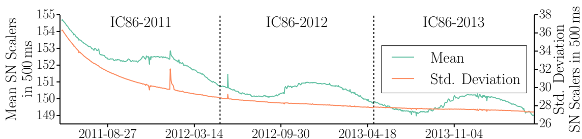
Figure 31. Mean and standard deviation of the supernova scaler distribution for the entire detector over the course of the first three years of the completed IceCube [46]. Spikes are due to calibration runs which injected light into the detector, and to fluctuations in individual DOMs.
