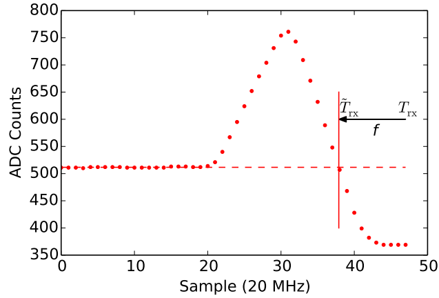
Figure 16. Digitized RAPCal pulse as received by a DOM, after cable dispersion. The zero-crossing of the baseline-subtracted pulse is used as a fine-delay correction f to the received timestamp T_{\text{rx}} .
