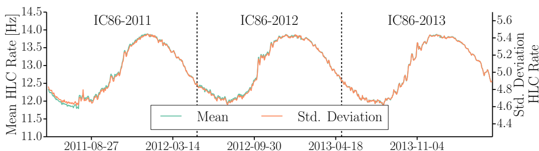
Figure 33. Mean and standard deviation of the local coincidence hit rate distribution [46]. Changes in dark noise rate do not contribute significantly to changes in the local coincidence hit rate, which is dominated by seasonal and weather-related changes in the atmospheric muon flux.
