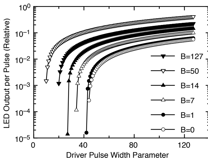
Figure 9. Light output from flasher LED pulses (relative to maximum), depending on brightness parameter ( B ) and width configuration parameters. Additional dynamic range is available by enabling from 1 to 12 individual LEDs per DOM.
