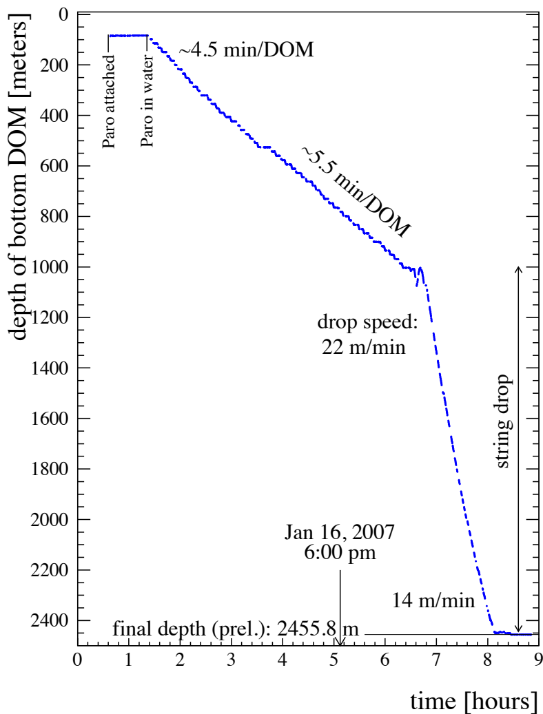
Figure 37. Depth of the lowermost DOM vs. time for String 48, deployed in the 2006–2007 season. The final depth is the preliminary Stage 1 depth measured during deployment (section 5.3.1), prior to the Stage 2 corrections derived from LED flasher measurements (section 5.3.2).
