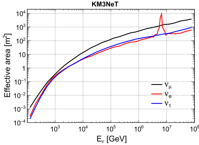
Figure 19. Effective areas of ARCA (two blocks) at trigger level for \nu_\mu , \nu_e , and \nu_\tau , as a function of neutrino energy E_{\nu} . The effective area is defined relative to an isotropic neutrino flux incident on the Earth, is averaged over both \nu and \bar{\nu} , and includes both NC and CC interactions. The peak at 6.3 PeV is due to the Glashow resonance of \bar{\nu}_e .
